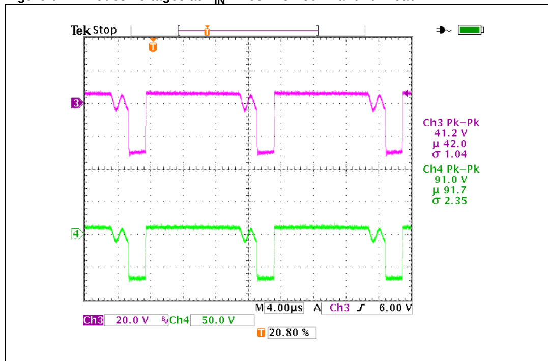
Figure 6. Diodes voltages at V_{IN} = 265VAC - 50Hz and full load
