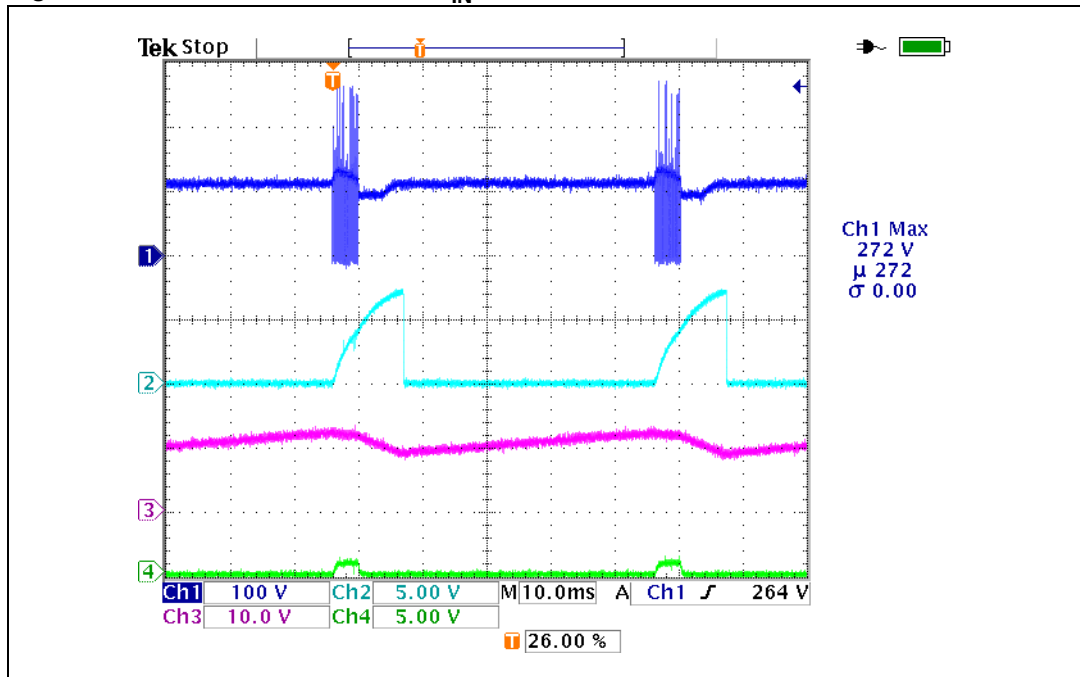
Figure 11. Short circuit on 5V at V_{IN} = 90VAC
