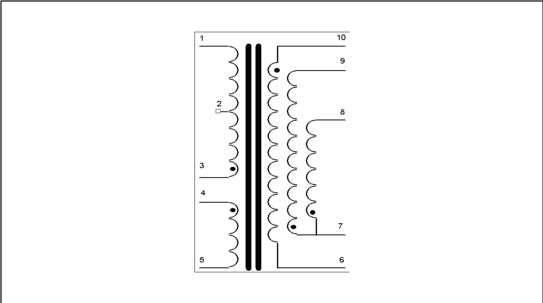
Figure 42. Transformer layout
