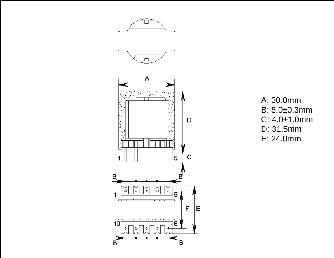
Figure 43. Dimension and appearance of transformer
