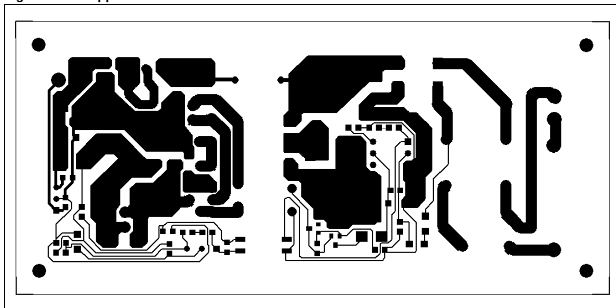
Figure 41. Copper tracks - bottom side
