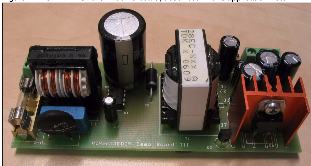
Figure 1. STEVAL-ISA023V1 demo board, described in this application note
